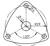
Plastic flange with mounting mechanism 20.045
