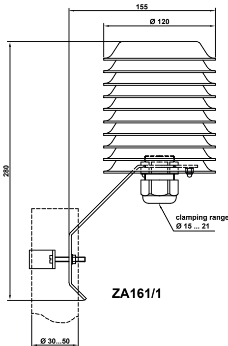
Console for wall mounting
